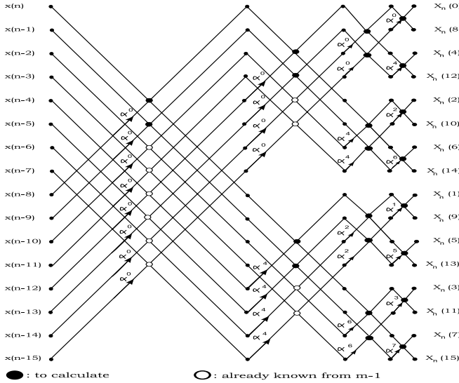
Fig. 2. Generalized Sliding FNT of N = 16 and P = 2
