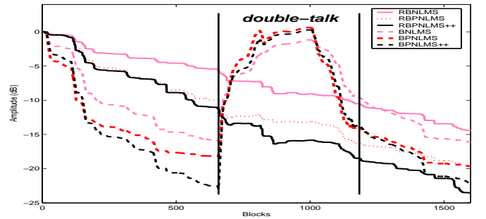
Fig. 6. Adaptation normalized misalignment
