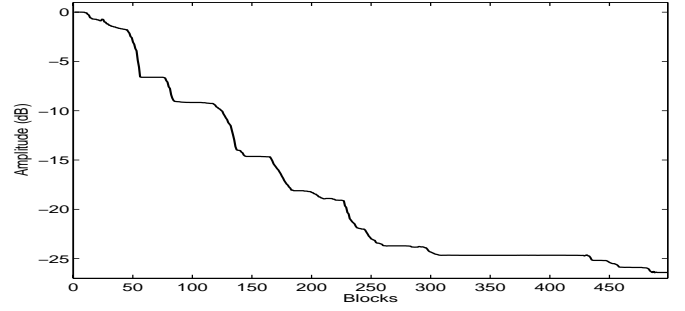
Fig. 4. Adaptation normalized misalignment
