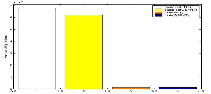
Fig. 5. Operations required for BPNLMS++ filtering for 10 blocks
