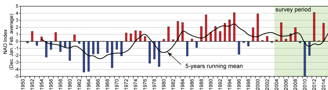
Figure 13. North Atlantic Oscillation Index (NAO) from 1950 to 2015 [47].
