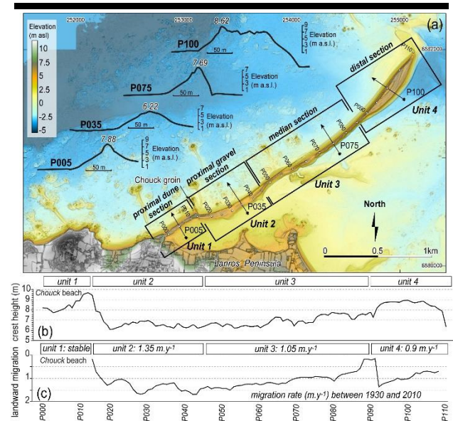
Figure 2. Morphological setting of the Sillon de Talbert. (a) Different longshore morphological units of the spit and representative beach profiles of the four units. (b) 2017 crest height. (c) Landward spit displacement in m \cdot y^{-1} between 1930 and 2010, after Stéphan, Suanéz, and Fichaut (2012), modified.
